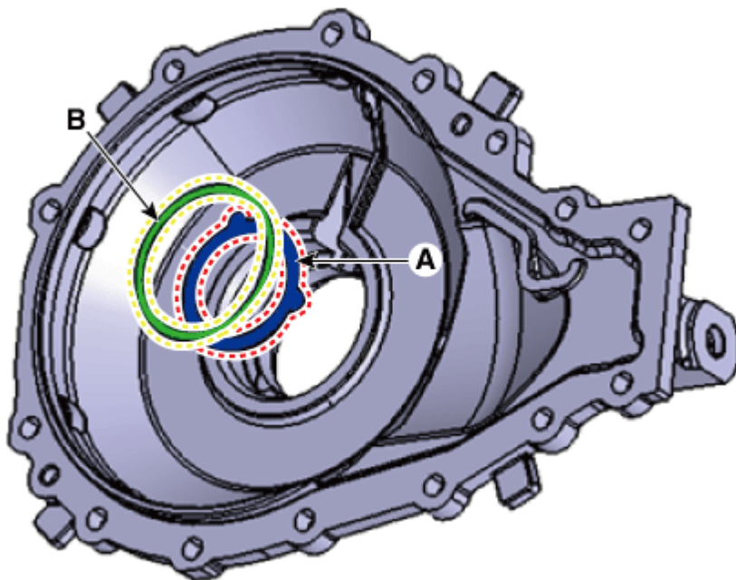
[Differential Case Side Cover]
